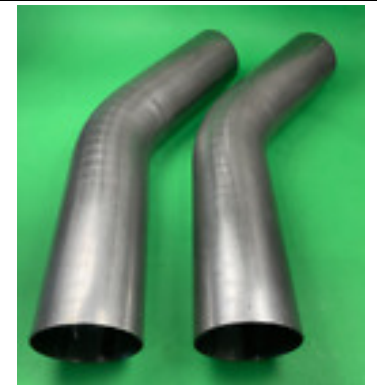
2 x 3"OD 30 Degree Exhaust Elbow Mandrel Bend 409 Stainless Steel 16 gauge
