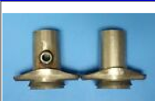
2.5"Ball Header To 2.5"OD Exhaust Pipe 2 Bolt Socket Collector With O2 Bung
