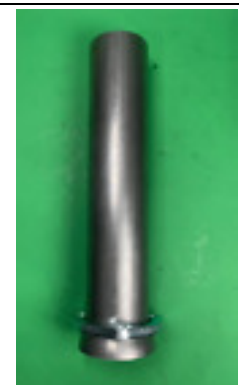
1 X 2.5"Ball Header To 2.5" 12"409 Stainless Socket 3 Bolt Collector Reducers
