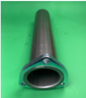
1 X 2.5"Header to 2.5"OD 12" 409 Stainless 3 Bolt Flange Gasket Style Collectors
