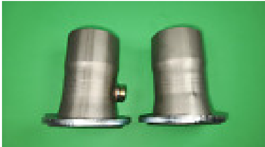
3.5"Header To 3"ID 409 Stainless 3 Bolt Flange Reducers With O2 Bung Made In USA
