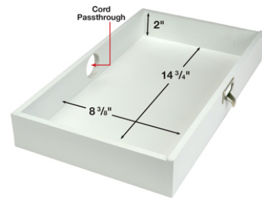
Drawer Dimensions
