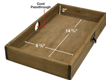
Drawer Dimensions
