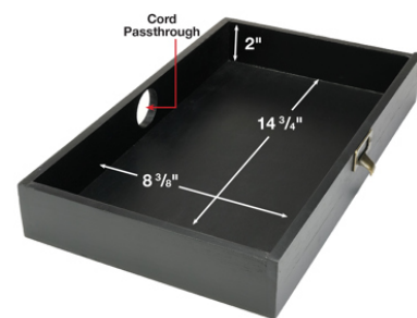
Drawer Dimensions
