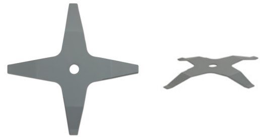
Mower blade AR17 for robotic mowers, 305 mm
